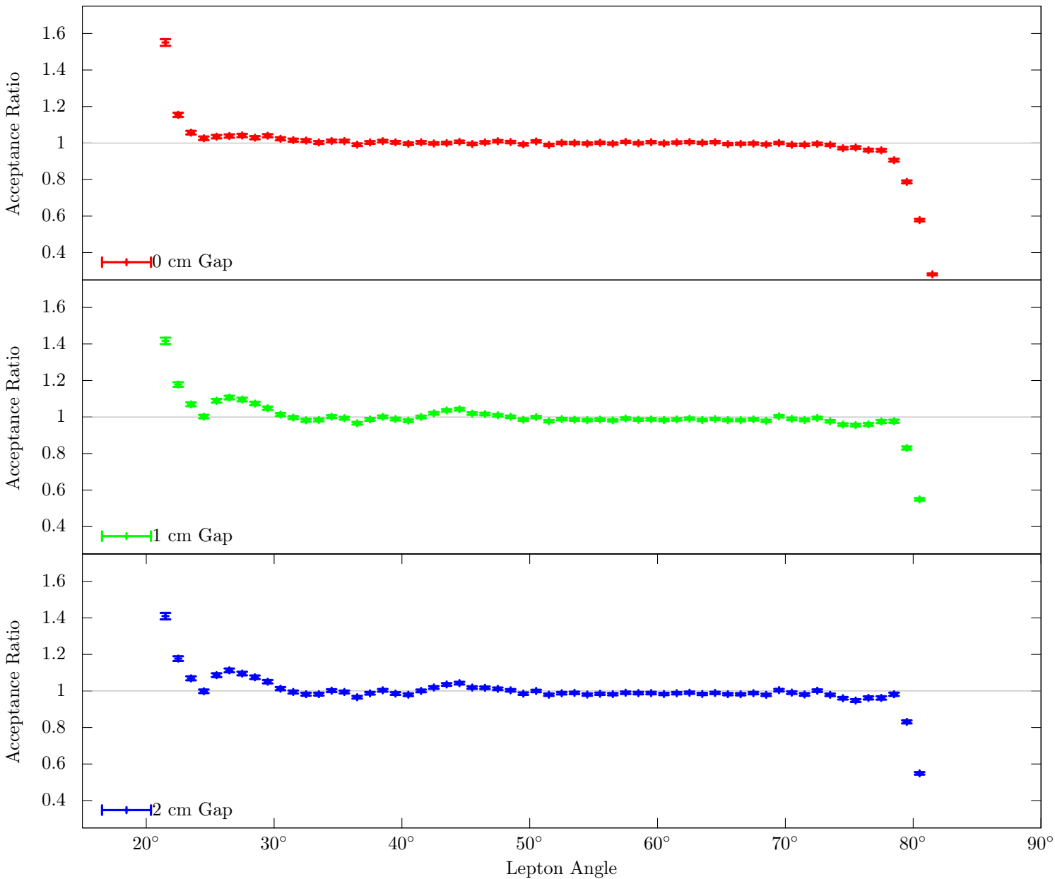
OLYMPUS Acceptance Ratios ( e^+/e^- )
