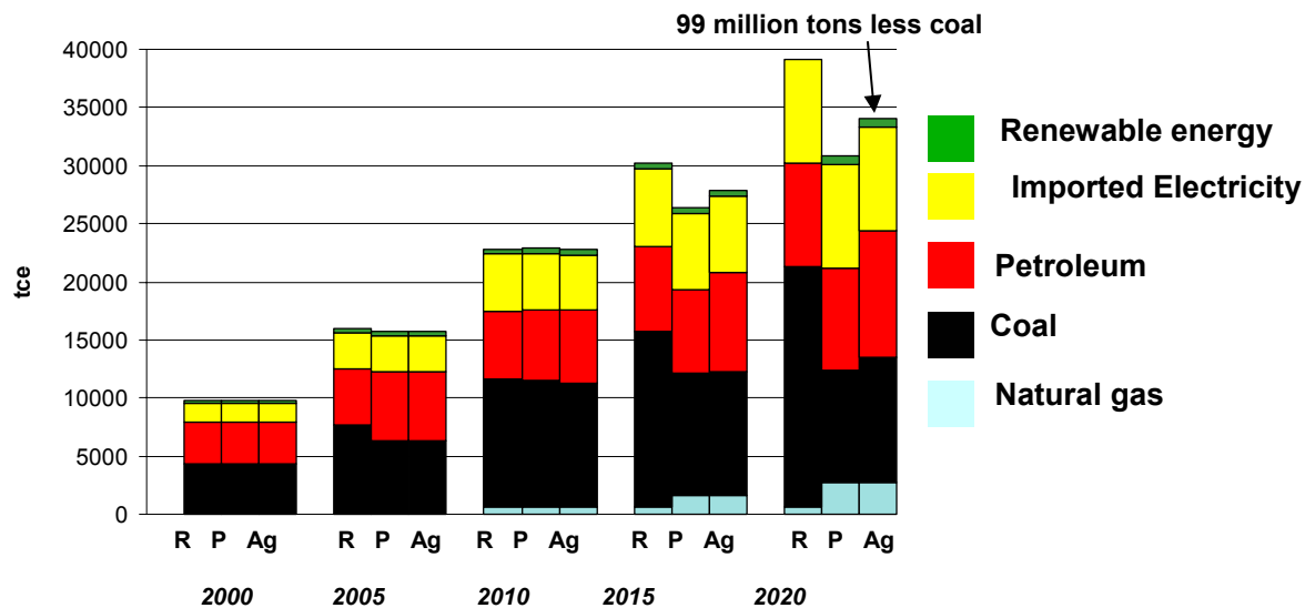
Figure 19: Energy Use in Guangdong Under Reference, Plausible, and Aggressive Scenarios
