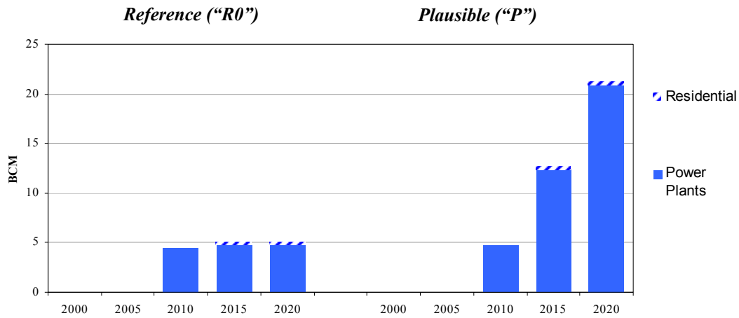
Figure 11: Natural gas consumption in Guangdong for reference and plausible SO 2 constraint scenarios
