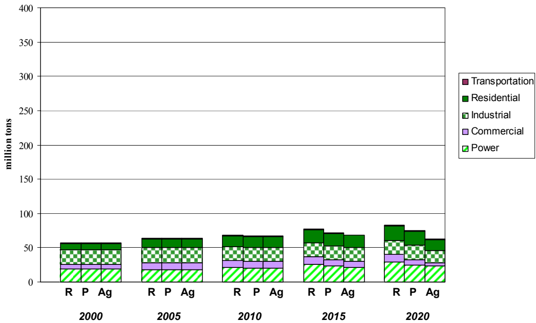
Figure 22: CO 2 Emissions from Beijing in the Reference, Plausible, and Aggressive Scenarios
