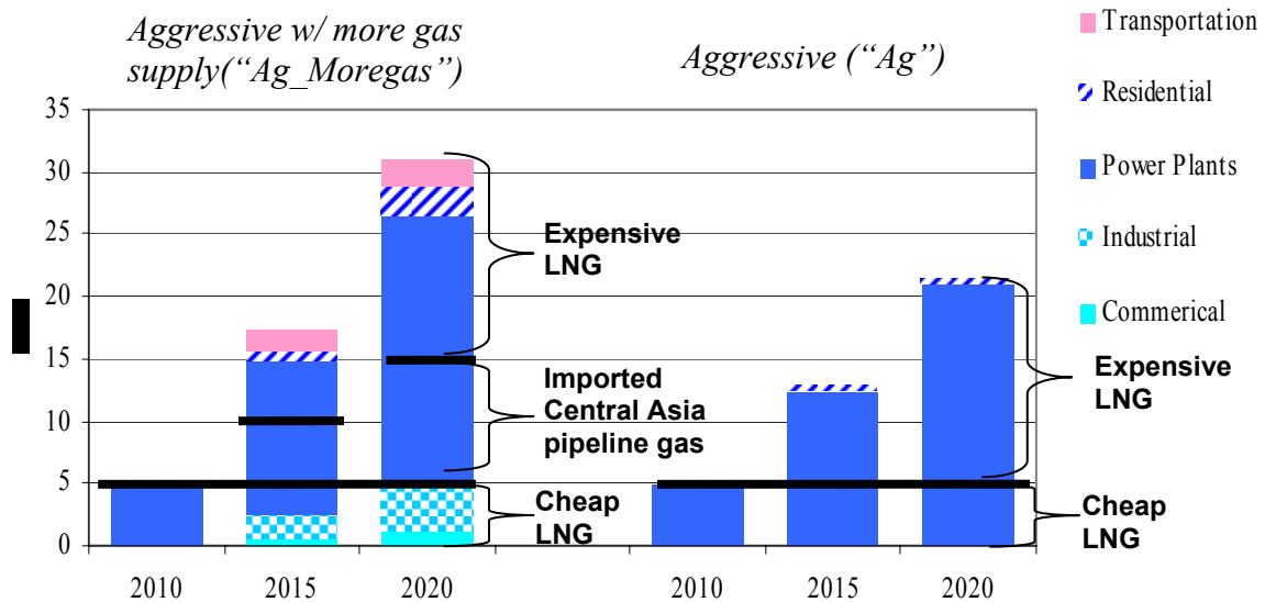
Figure 18: Gas Supply Options for Guangdong and Natural Gas Demand by Sector
