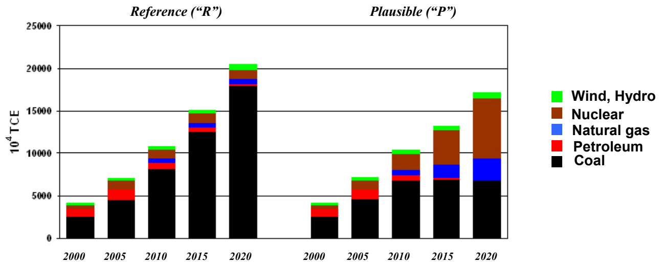
Figure 12: Fuel consumption in Guangdong Power Sector for reference and plausible SO 2 constraint scenarios
