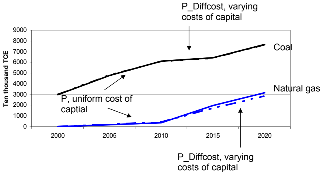
Figure 17: Coal and Natural Gas Consumption in the Shanghai (Power Sector)
