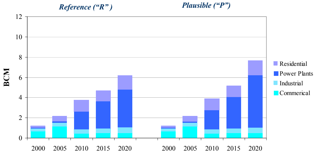
Figure 9: Natural gas consumption in Beijing for reference and plausible SO 2 constraint scenarios
